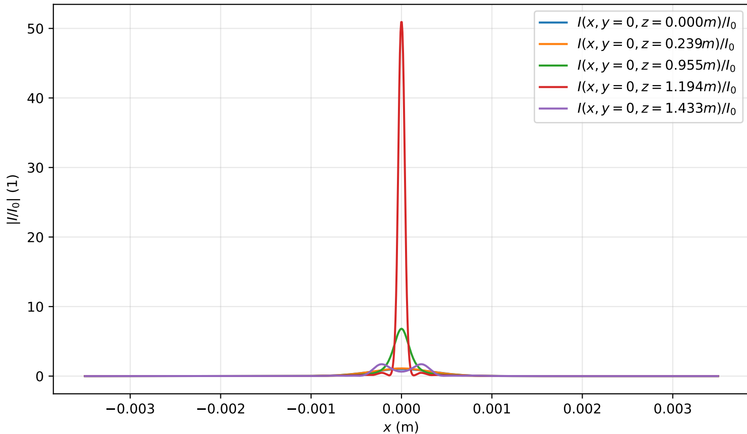
Intensity profile I(x, y = 0, z)/I_0 , \text{Pin}=2.0\text{Pcr} , artificial time
